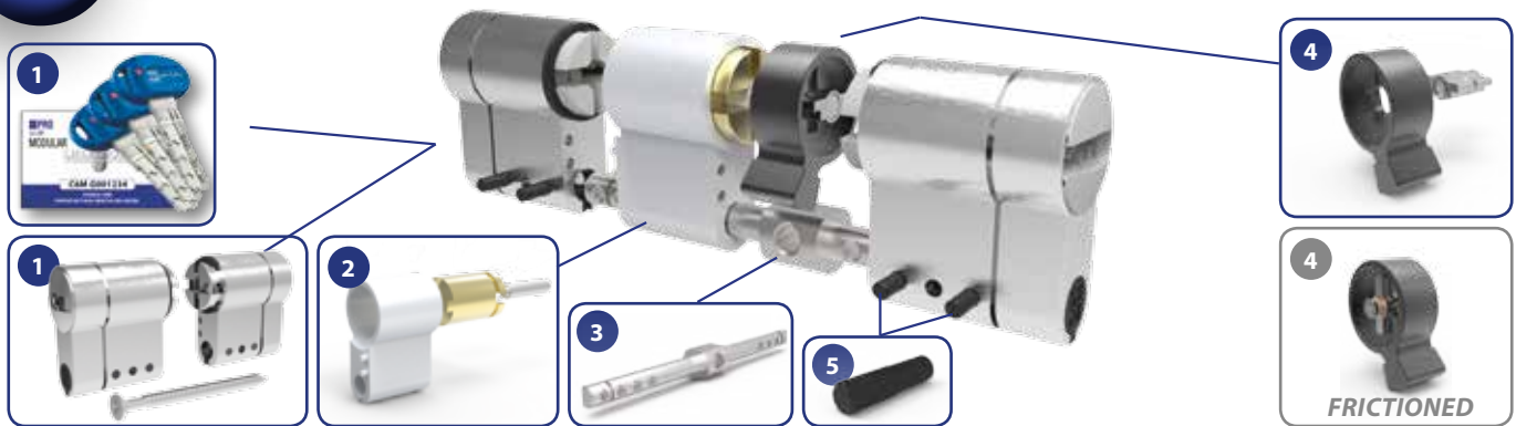
EXAMPLE - DOUBLE CYLINDER - KEY/KEY - Measure 31-51 (82) (FRICTIONED)
