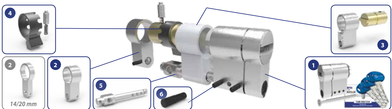
EXAMPLE - HALF CYLINDER FOR 30 mm THICKNESS LOCKS - Measure 51 (66) (14/20 mm THICKNESS LOCKS)
